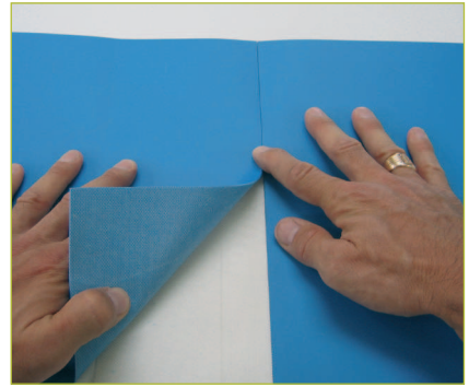
PE Straight or diagonal step overlap
